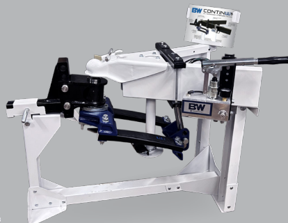
CONTINUUM HITCH STAND WDXA8049 *Hitch sold separately
